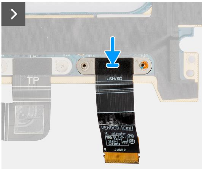
2x M1.4x1.2
