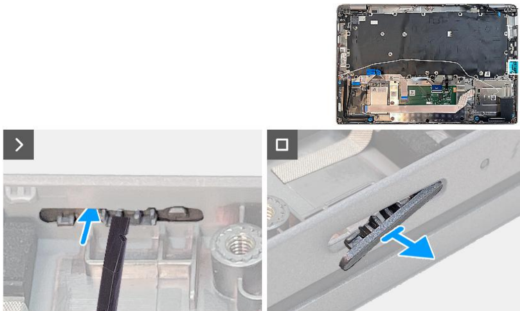
Figure 65. Removing the dummy SIM-card slot filler
