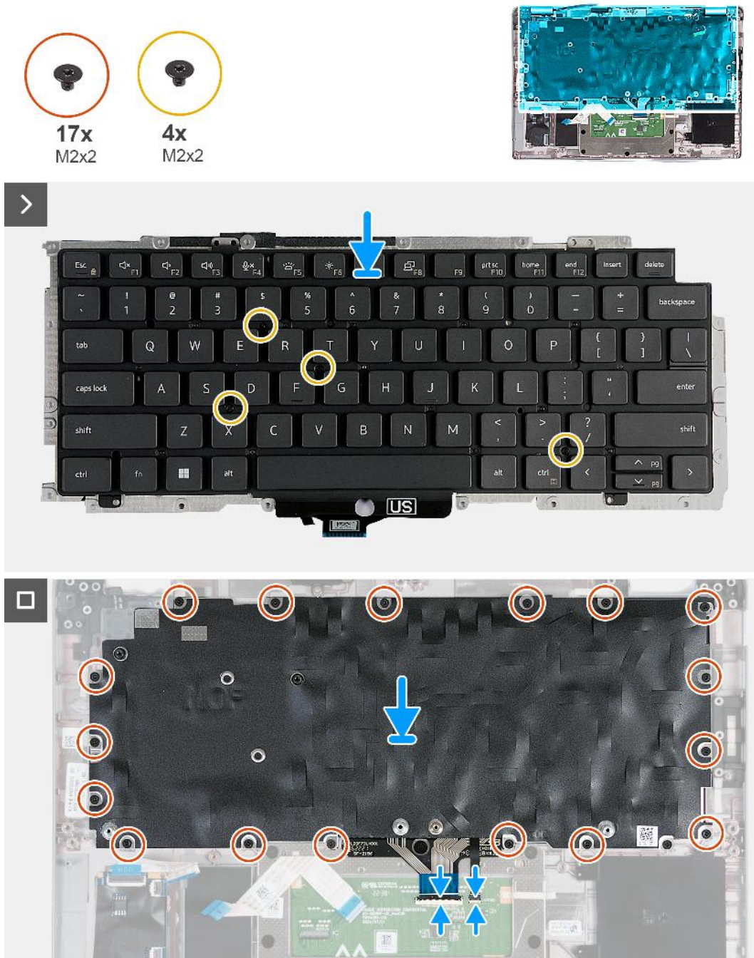
Figure 62. Installing the keyboard
