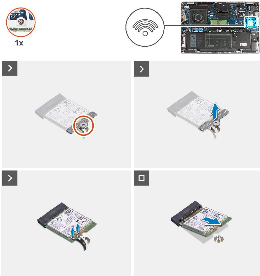
Figure 10. Removing the wireless card
