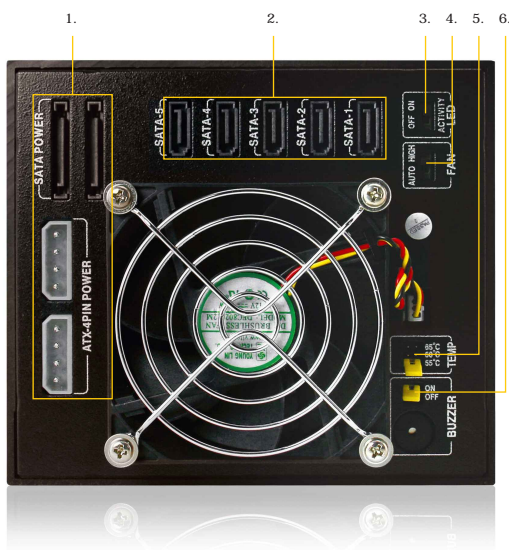
Rear view IB-555SSK
